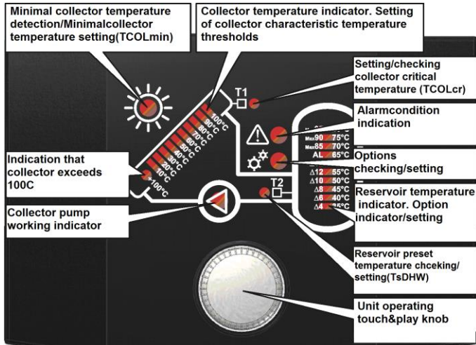
Fig. 5.1 Controller screen
