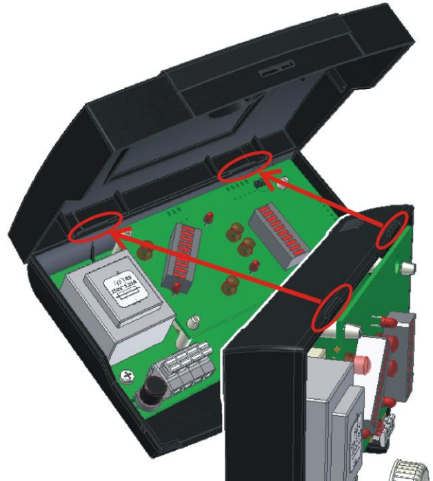
Fig. 13.1 Casing closing first step
