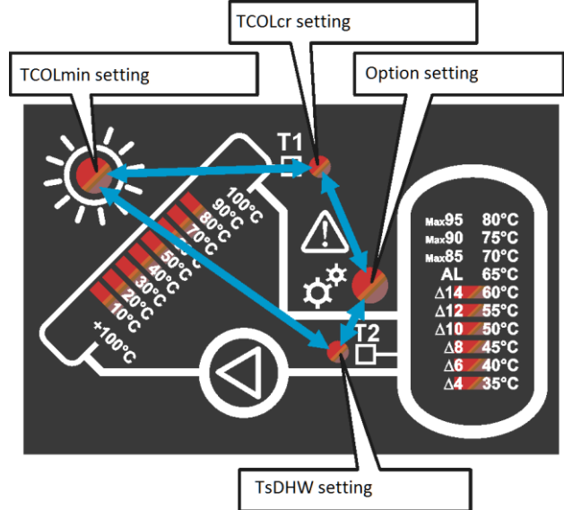
Fig. 5.4 Screen navigation.
